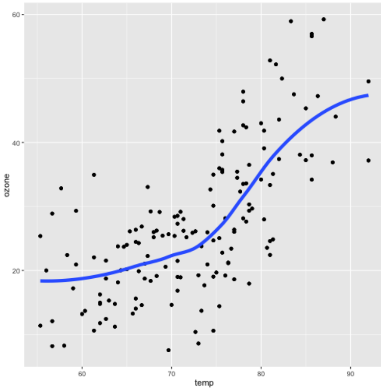
Loess Smoother for Ozone and Temperature
