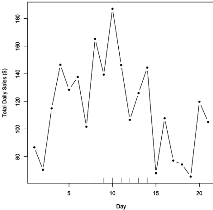
More Realistic Daily Sales Data
