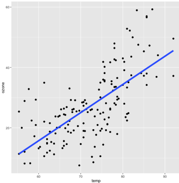
Linear Model for Ozone and Temperature
