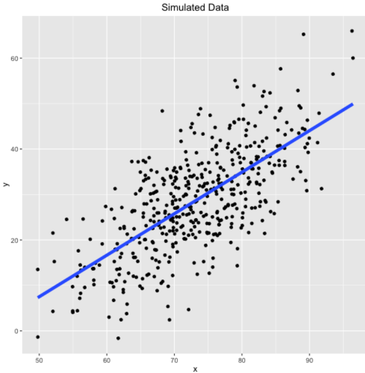
Simulated Data with a Linear Model
